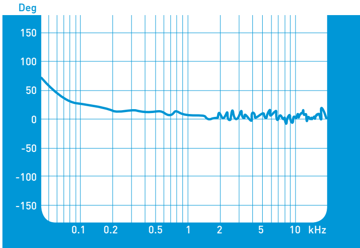
Phasengang, C120-Coax + CB120
